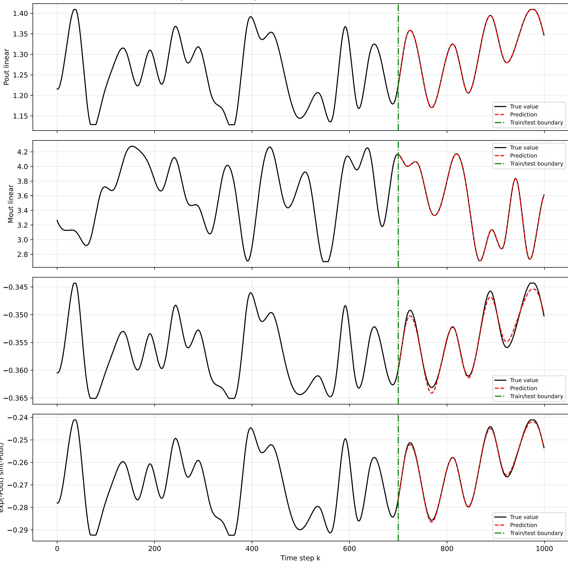
Koopman + Solverz prediction (RMSE = 4.1173e-04)
