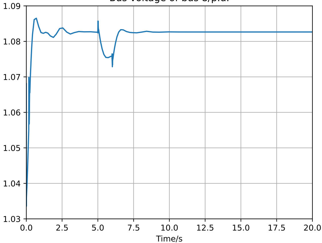
Bus voltage of bus 8/p.u.
