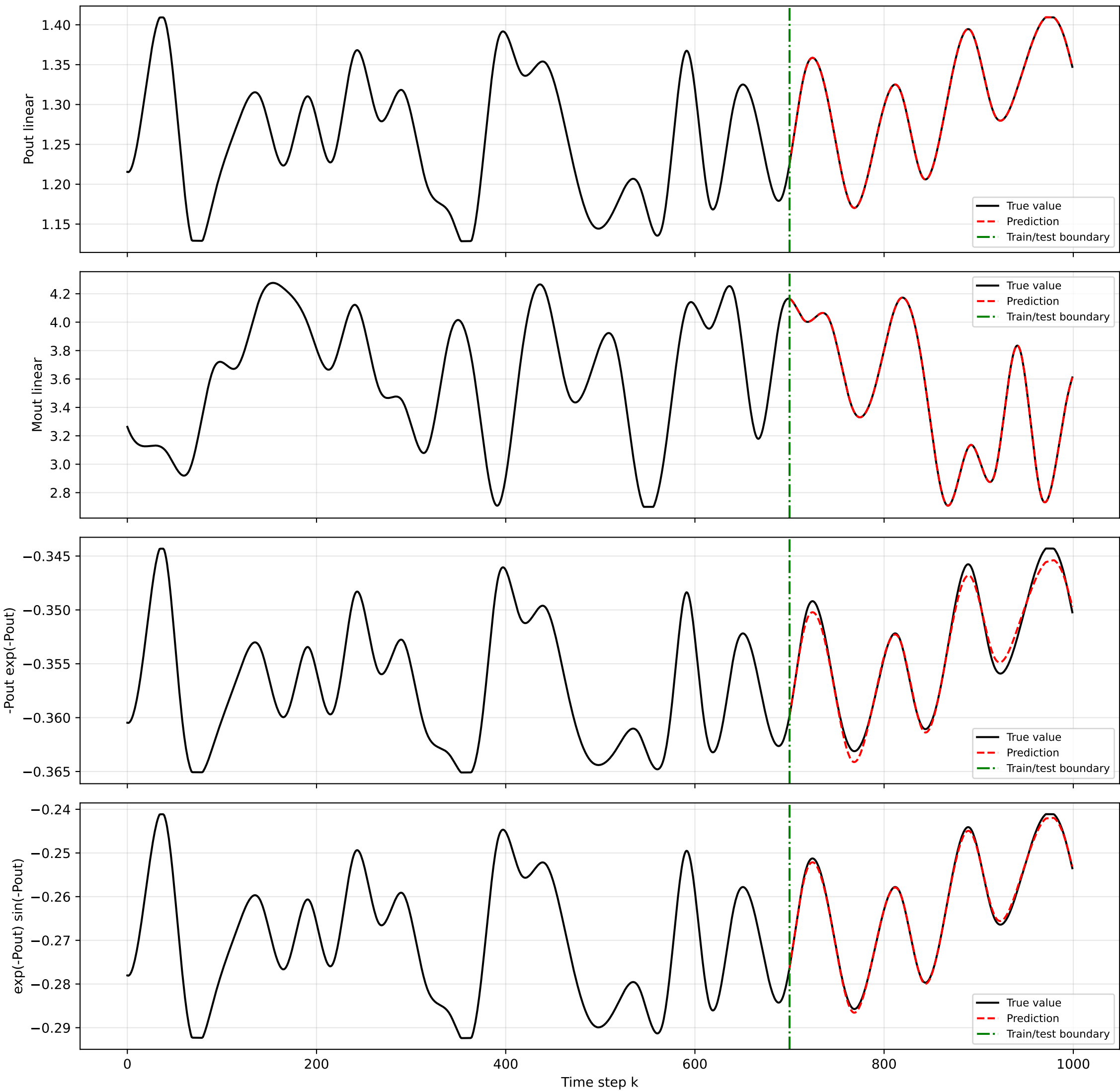
Koopman + Solverz prediction (RMSE = 4.1173e-04)
